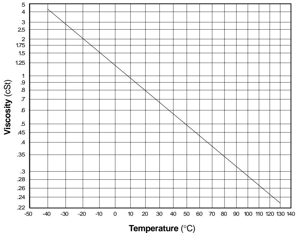
Fluorinert Liquid FC-3283 Viscosity (cSt) vs. Temperature (°C)
